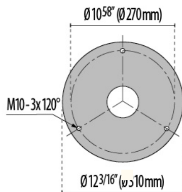
Base Details
